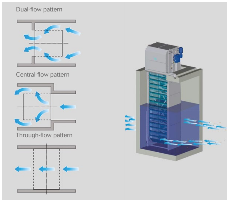
Band Screen Flow Patterns
